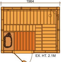
2020MS INT. VOL. 6.32 m 3 SCA 6.0 KW
