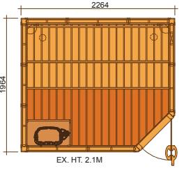
2023RSC INT. VOL. 7.37 m 3 SCA 8.0 KW
