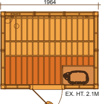
2020RL INT. VOL. 6.32 m 3 SCA 6.0 KW
