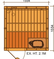
1620LSC INT. VOL. 4.88 m 3 SCA 6.0 KW
