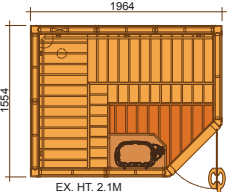
1620RLC INT. VOL. 4.90 m 3 SCA 6.0 KW
