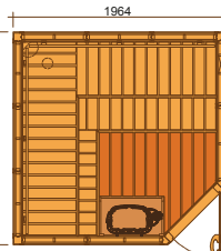
2023LSC INT. VOL. 7.37 m 3 SCA 8.0 KW
