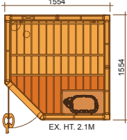
1620MS INT. VOL. 4.88 m 3 SCA 6.0 KW
