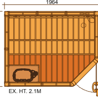
2020LL INT. VOL. 6.32 m 3 SCA 6.0 KW
