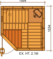
1620RL INT. VOL. 4.88 m 3 SCA 6.0 KW
