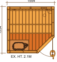
1620LL INT. VOL. 4.88 m 3 SCA 6.0 KW
