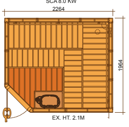
2023LLC INT. VOL. 7.37 m 3 SCA 8.0 KW
