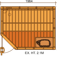
2020MD INT. VOL. 6.32 m 3 SCA 6.0 KW
