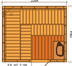
2023RL INT. VOL. 7.37 m 3 SCA 8.0 KW
