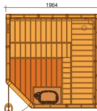
2020LLC INT. VOL. 6.32 m 3 SCA 6.0 KW
