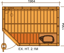
1616LL INT. VOL. 3.77 m 3 SCA 4.5 KW
