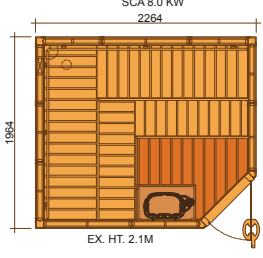
2023RLC INT. VOL. 7.37 m 3 SCA 8.0 KW
